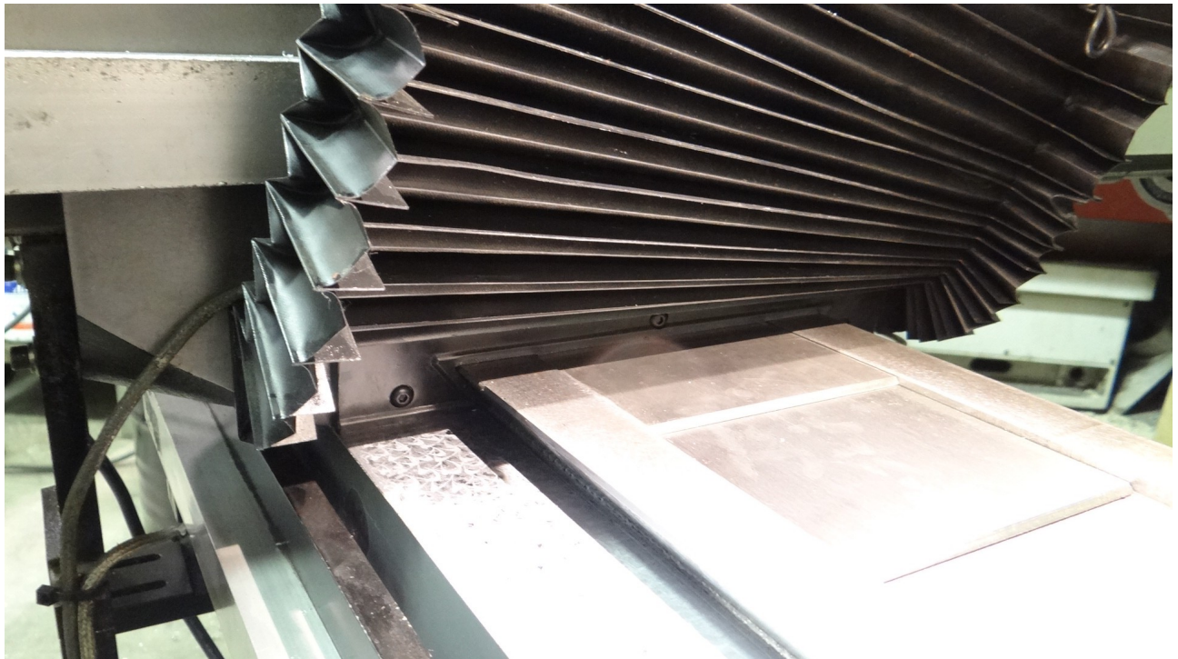
Way covers attach to existing saddle wiper cover plates
