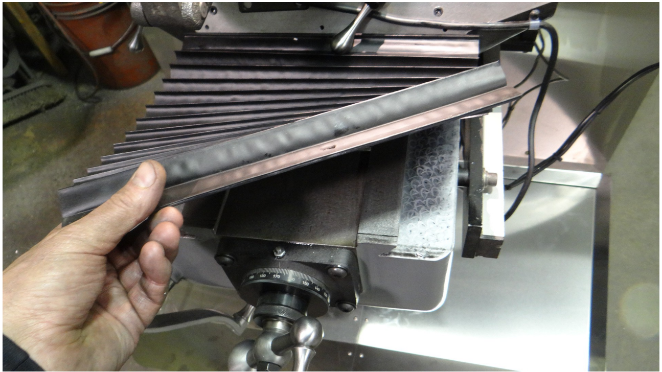
EZ lift off front section way cover for EZ clean up
